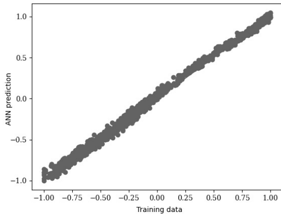
Figure 5: Comparison of the ANN’s trained prediction against the training output data
